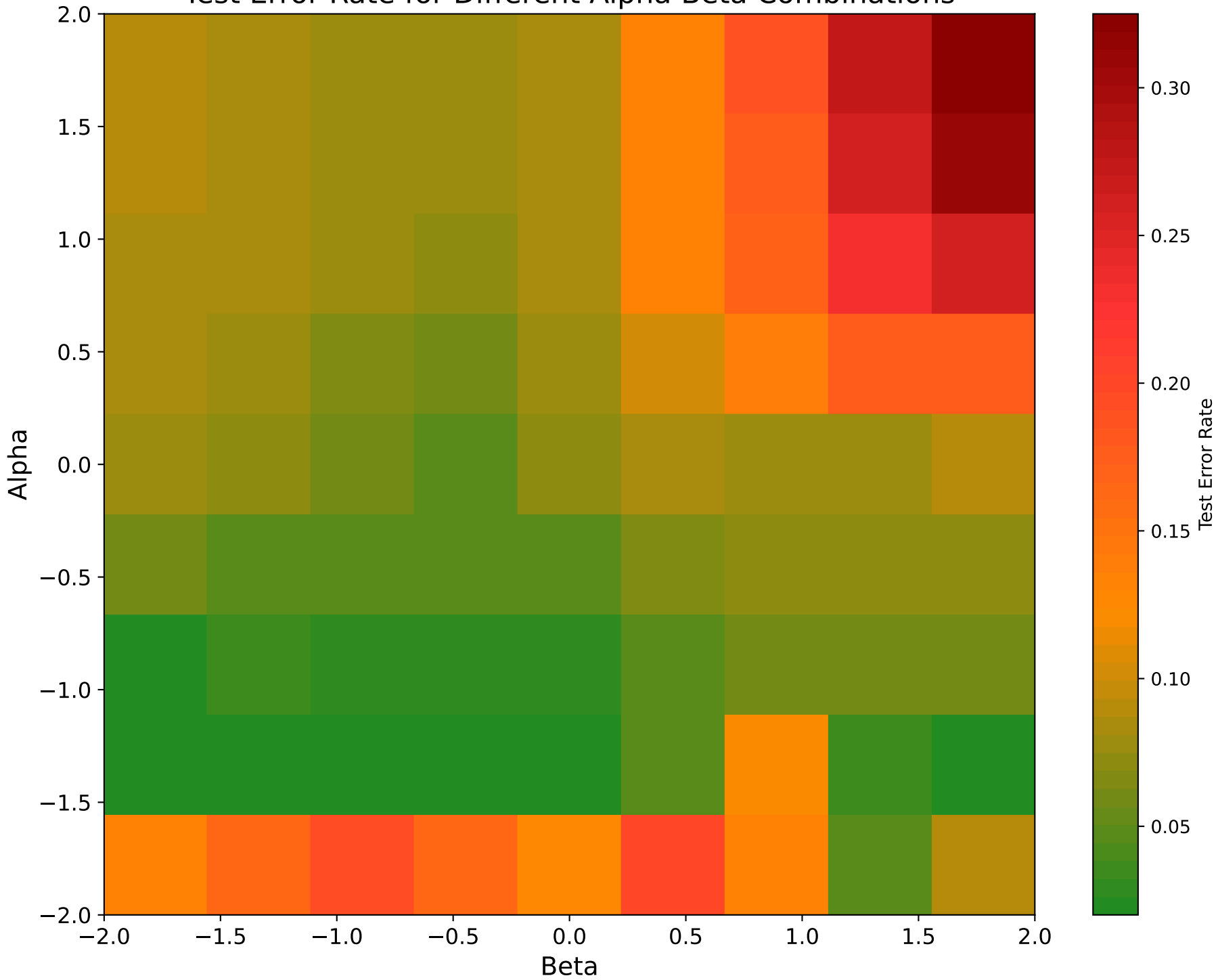
Test Error Rate for Different Alpha-Beta Combinations
